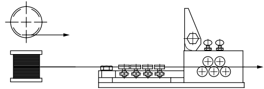
Right Hand Straightener Horizontal Spool
