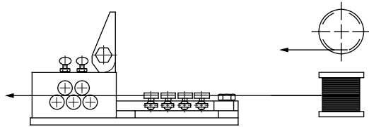
Left Hand Straightener Horizontal Spool
