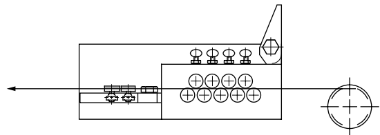
Right Hand Straightener Vertical Spool
